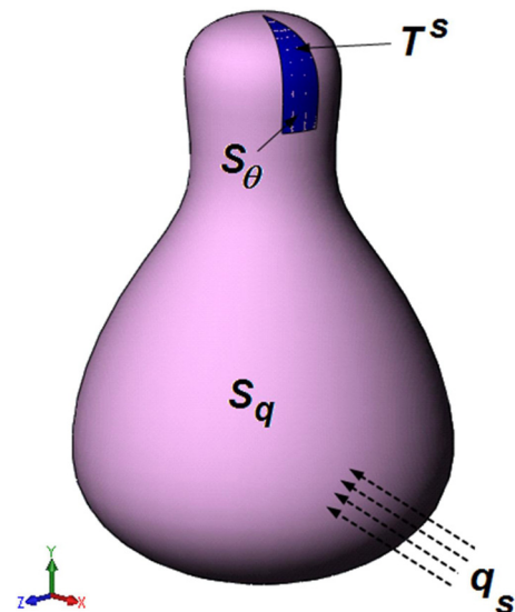
Fig. 1. Body subjected to heat transfer.
