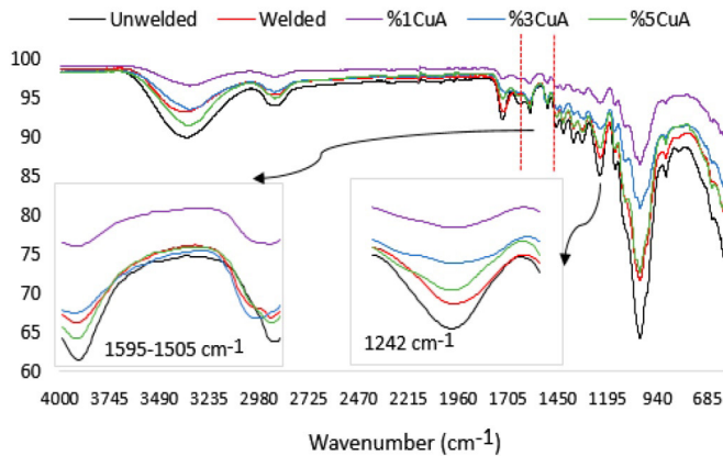
Figure 4: FTIR spectra of welded and control wood.
