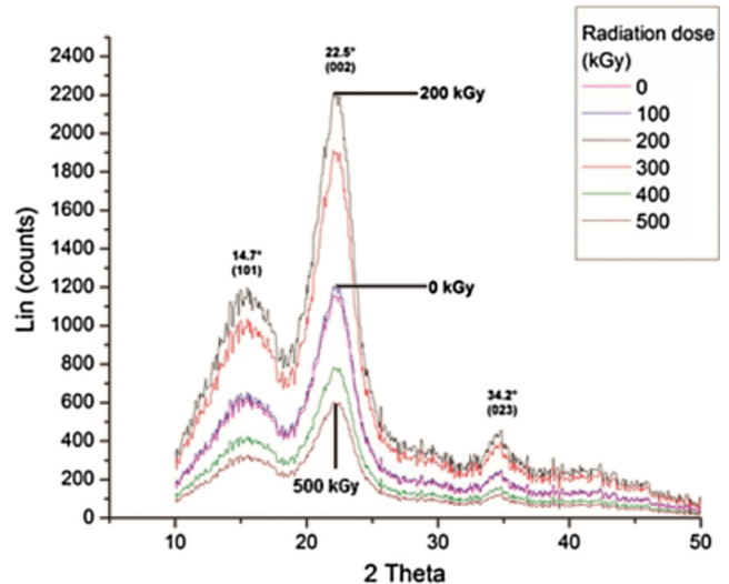
Fig. 3. X-ray diffraction pattern of cellulose.
