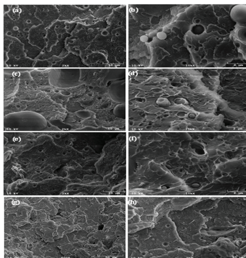
Fig. 4: SEM pictures of the composites. a,b) pure SMA; c,d) SMA/starch blends; e,f) SMA/AC blends; g,h) SMA/UFC blends.
