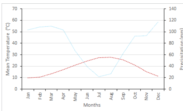
Figure 2. Ombrothermic diagram of Dörtöl Meteorological Station, Hatay. Blue dashed line represents monthly total precipitation and red dashed line represents mean monthly temperature values (1960-2010)
