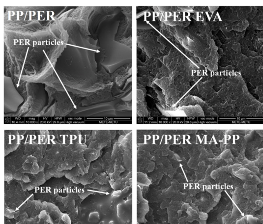
Figure 6. SEM micro-images of composites.
