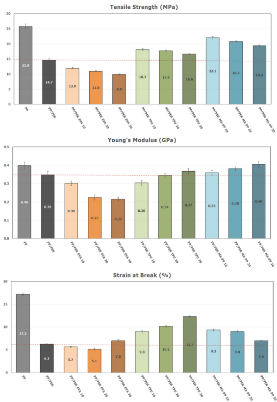
Figure 4. Tensile test data of samples.
