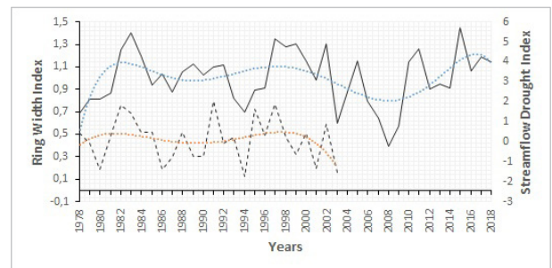
Figure 11 Mean Ring-Width Index Chronology (RWI) (Solid Line) and 3-Month Streamflow Drought Index ( SDI_3 ) for July–September (Dashed Line). Dotted Lines Show the Polynomial Trendline of Each Graphic. Correlation Coefficient between RWI and SDI_3 is .51 ( p < .05 )
