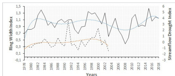
Figure 10 Mean Ring-Width Index Chronology (RWI) (Solid Line) and June's Streamflow Drought Index ( SDI_1 ) (Dashed Line). Dotted Lines Show the Polynomial Trendline of Each Graphic. Correlation Coefficient between RWI and SDI_1 is .51 ( p < .05 )
