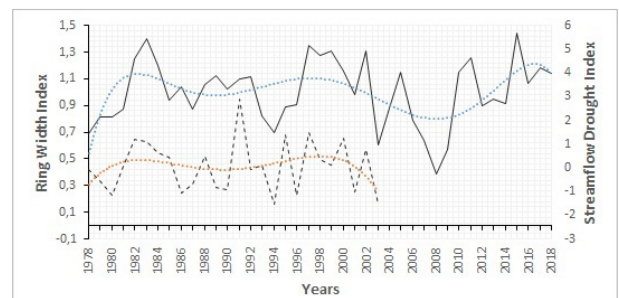
Figure 12 Mean Ring-Width Index Chronology (RWI) (Solid Line) and 3-Month Streamflow Drought Index ( SDI_3 ) for June–August (dashed line). Dotted Lines Show the Polynomial Trendline of Each Graphic. Correlation Coefficient between RWI and SDI_3 is .57 ( p < .01 )
