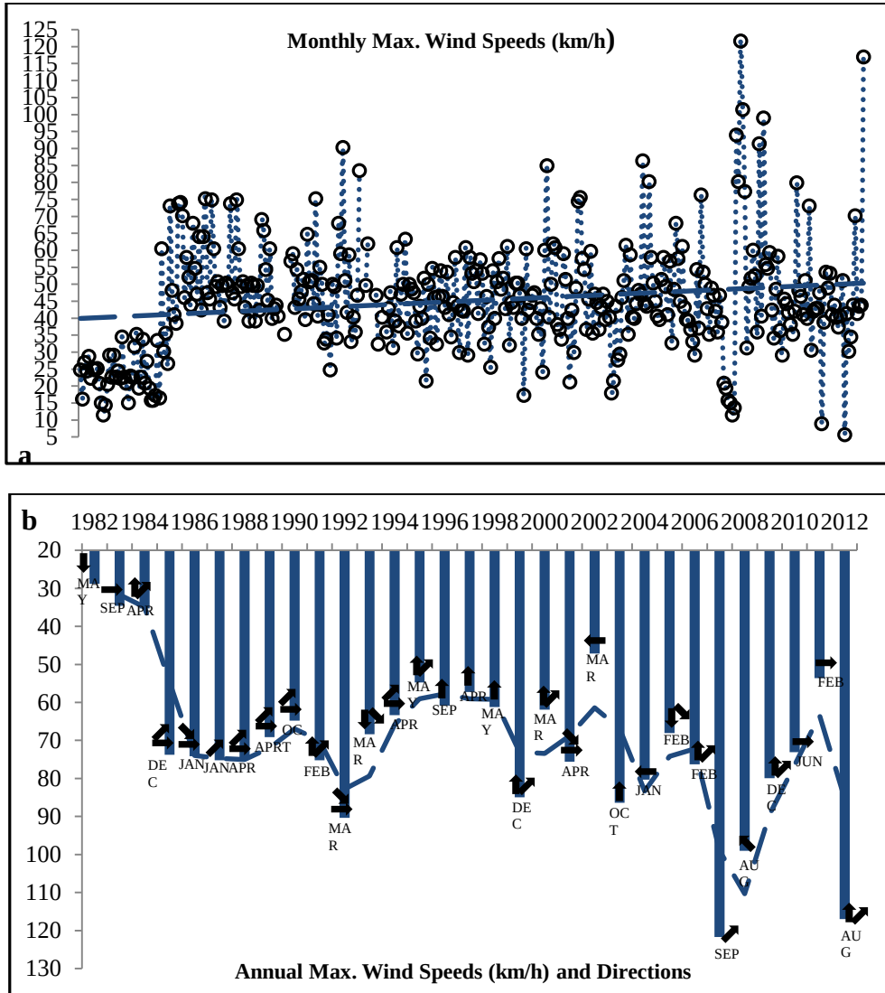
Figure 3. Monthly maximum wind speeds (a). Annual maximum wind speeds (km/h) and directions (b) between 1982 and 2012.
