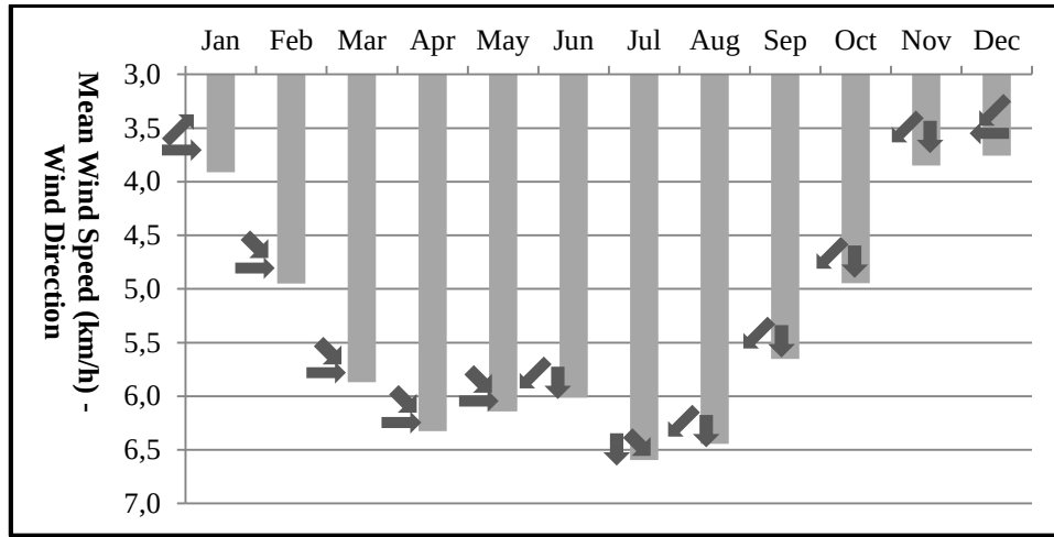
Figure 2. Monthly mean wind speeds (km/h) together with their weighted directions.
