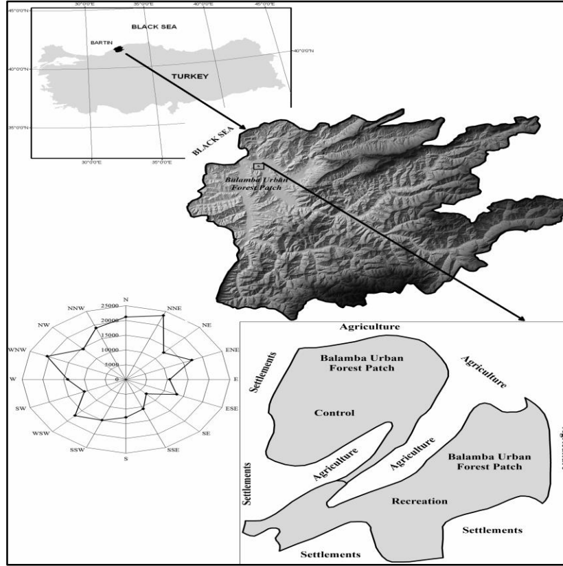
Figure 1. Location of the Balamba Urban Forest Patch within Bartın watershed of Turkey. Wind directions based on the number of blows (TSMS, 2013).
