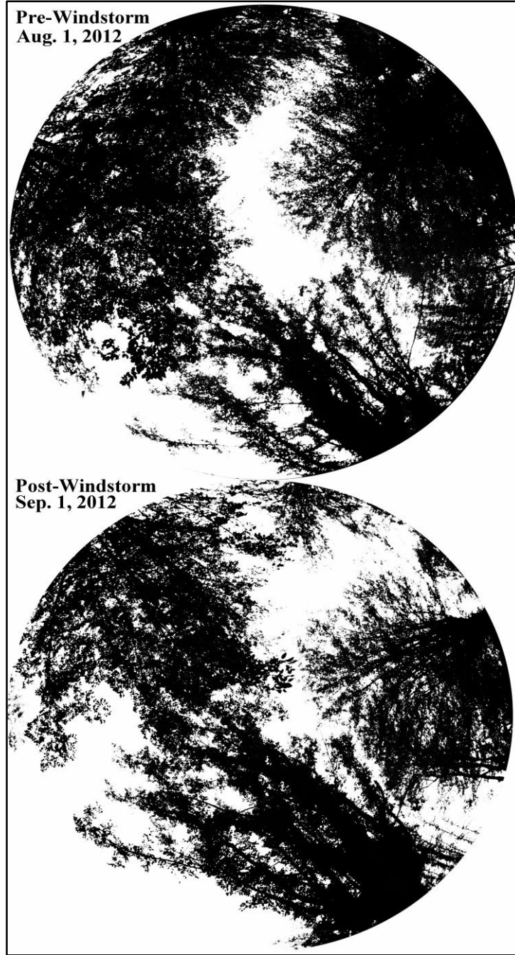
Figure 4. Sample hemispherical photos of the first photographing point (recreation) indicating the pre- (Aug. 1 st , 2012) and post-windstorm (Sep. 1 st , 2012).
