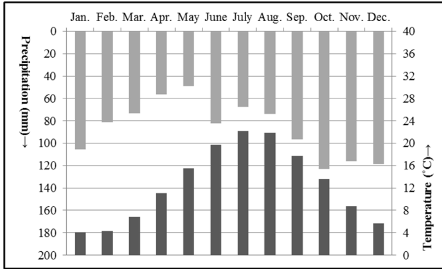
Figure 2. Mean monthly total precipitation data (left-grey bars-downwards). Mean monthly temperature data (right-dark bars-upwards).
