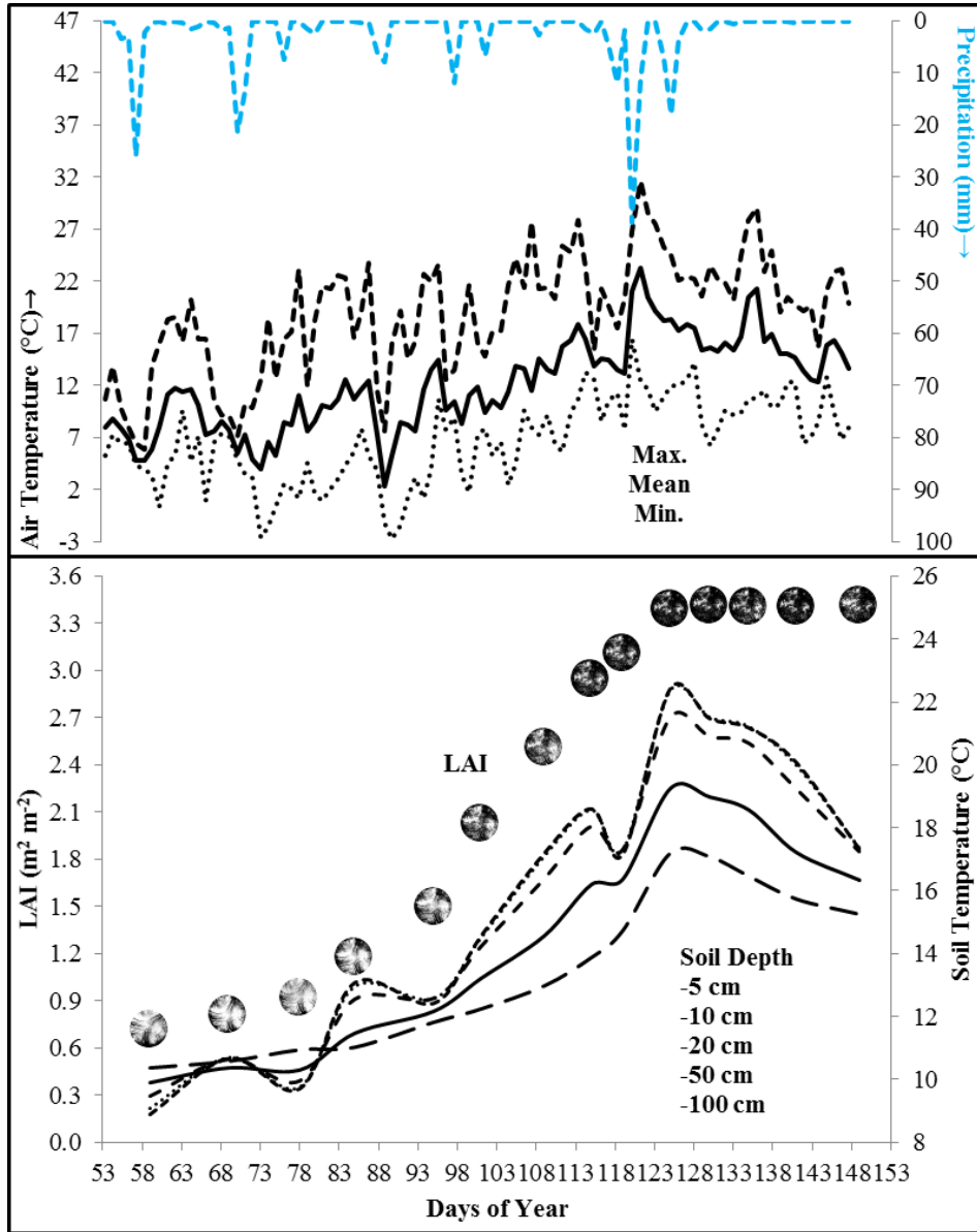
Figure 3. Daily maximum, mean and minimum air temperatures and precipitation (above), LAI and mean soil temperatures of different depths (below) along the monitoring period.
