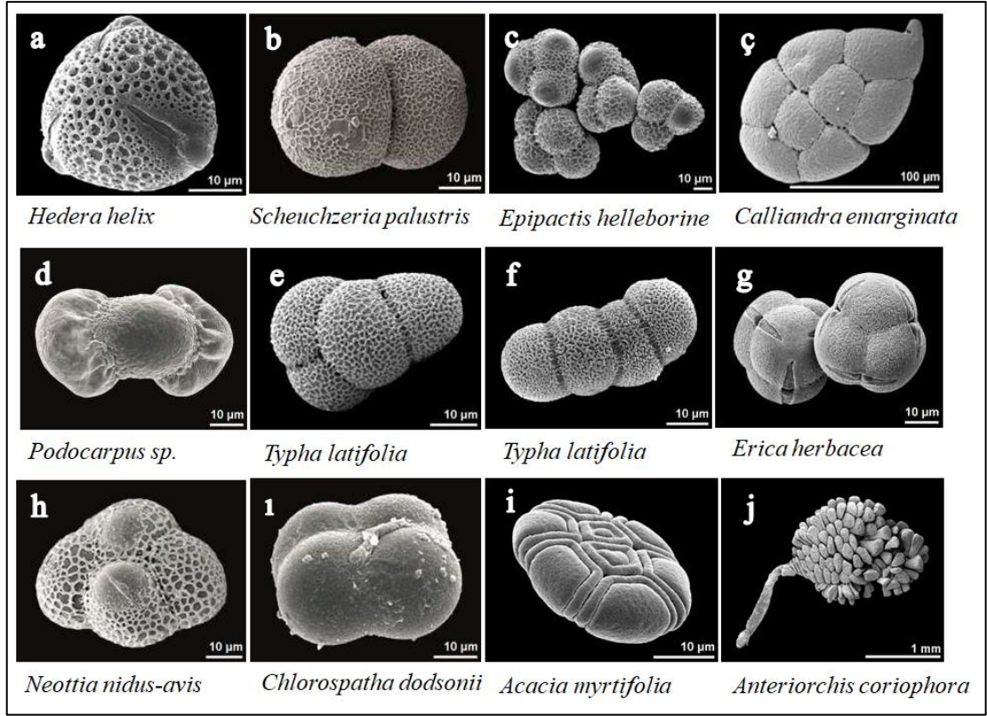
Şekil 1: Polen tipleri Monad (a), diyad (b), tetrad (c), poliyad (ç), vesikulat/sakkat (d), T şekilli tetrad (e), linear tetrad (f), tetrahedral tetrad (g), desukkat tetrad (h), tetragonal tetrad (ı), massula (i) ve polinyum (j) (Hesse vd., 2009; Paldat, 2015)
